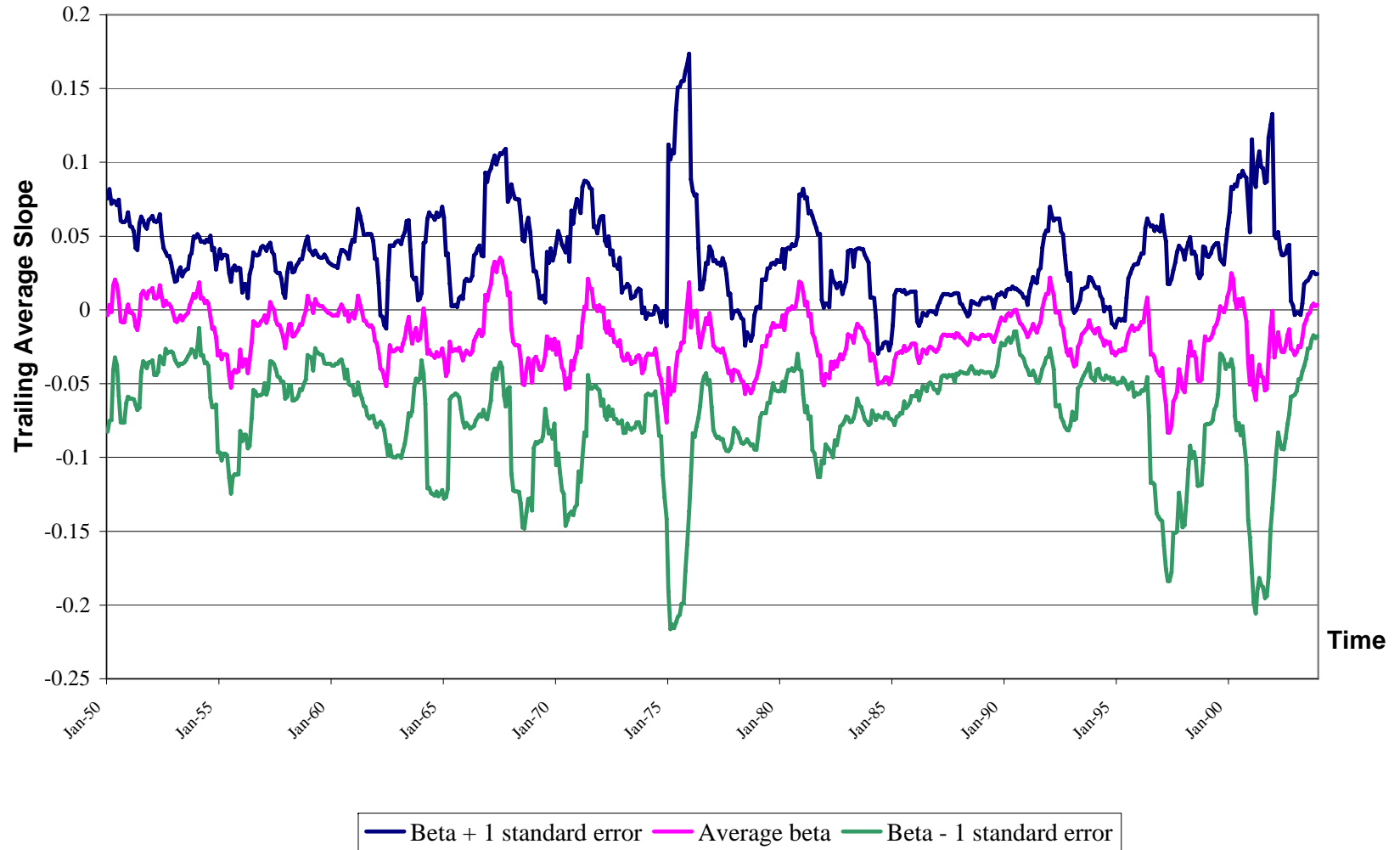
Figure 2 Trailing average slope coefficient from the regression the of one-month return on ISSUE (-6, -17)
