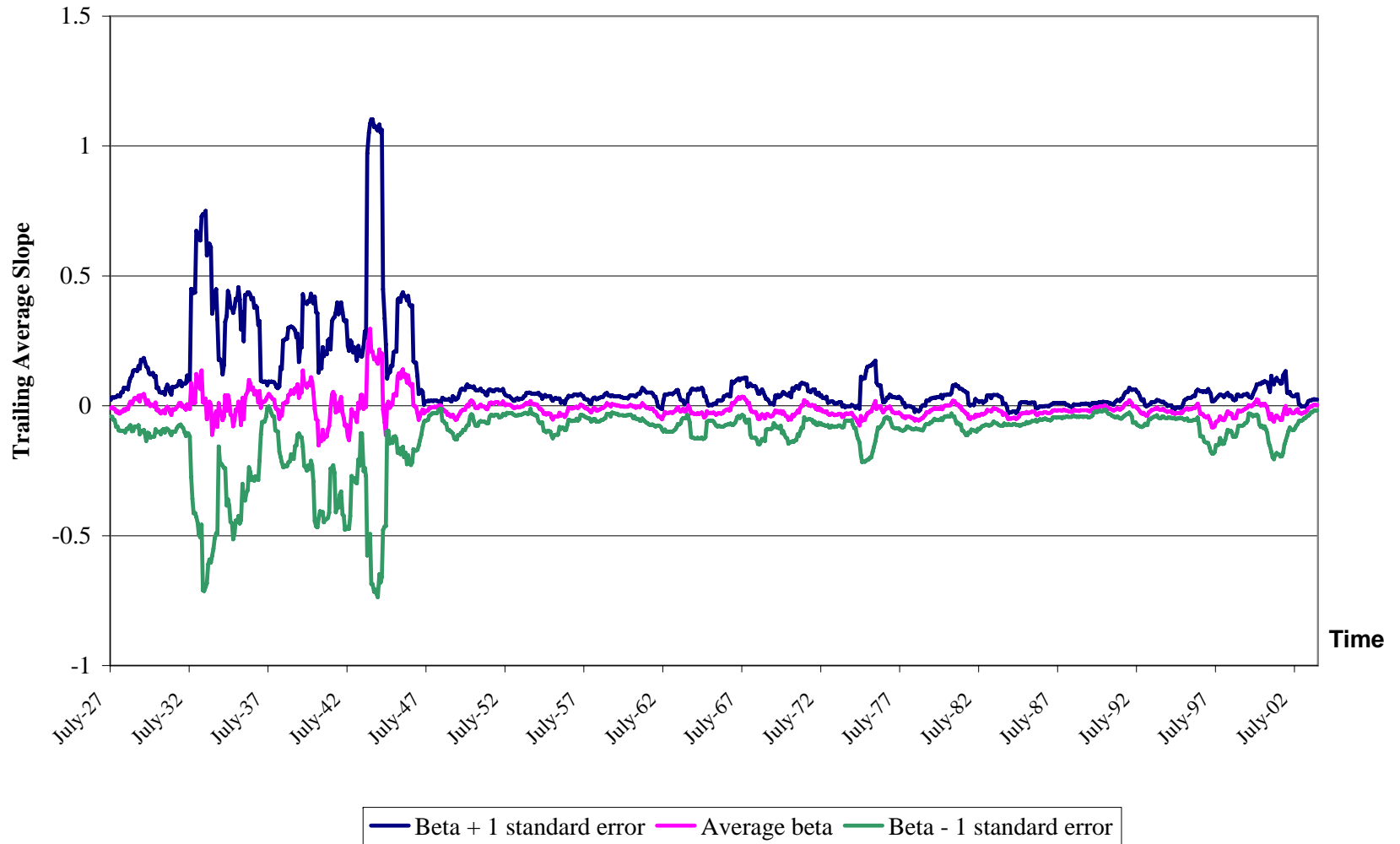
Figure 1 Trailing average slope coefficient from the regression of the one-month return on ISSUE (-6, -17)
