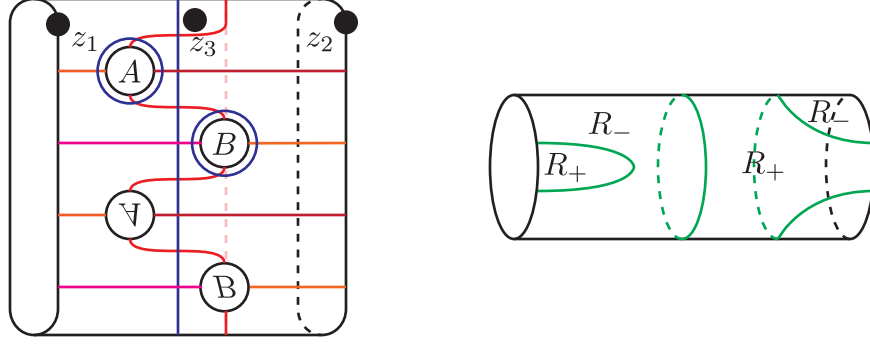
FIGURE 3. The diagram \text{TC}_0(\mathcal{Z}) and the corresponding bordered-sutured manifold. Left: the genus 1 case of the diagram \text{TC}_0(\mathcal{Z}) . Right: the corresponding sutures on [0, 1] \times S^1 \subset \partial([0, 1] \times F^\circ(\mathcal{Z})) .
