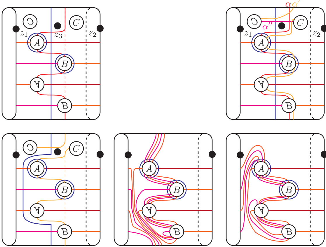
FIGURE 4. Exact triangle for TC_0(\mathcal{Z}) . Top left: the bordered-sutured Heegaard diagram TC_0(\mathcal{Z}) with an extra handle. Top right: the bordered-sutured triple diagram inducing the exact triangle in Theorem 13. Bottom: Identifying the third term in the exact triangle with the positive boundary Dehn twist. The bottom left and bottom center differ by a sequence of handleslides and a destabilization; the bottom right is obtained by applying a surface diffeomorphism to the bottom center.
